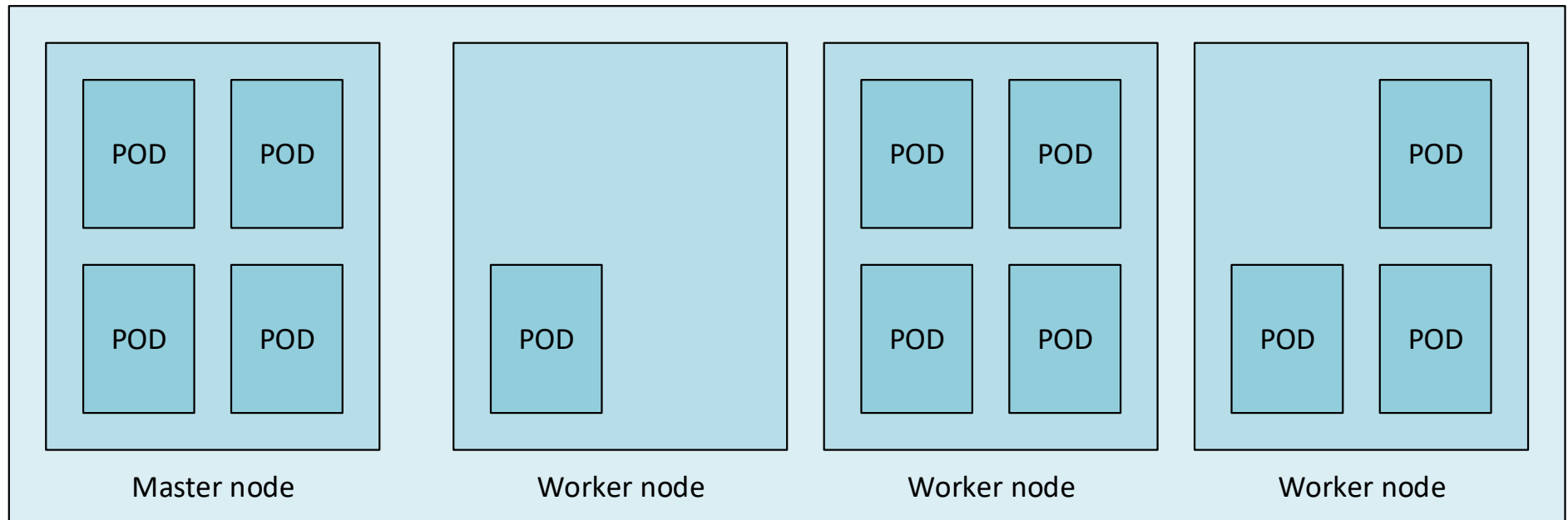
Kubernetes cluster
